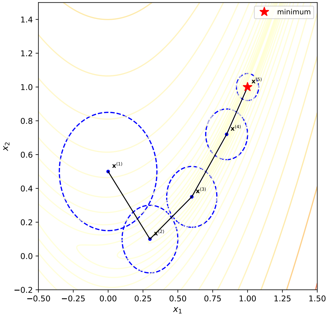
Trust Region Method on Rosenbrock
