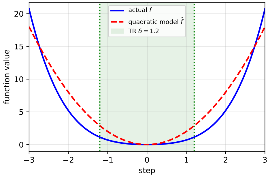
Poor model: \eta < \eta_1 (shrink TR)
