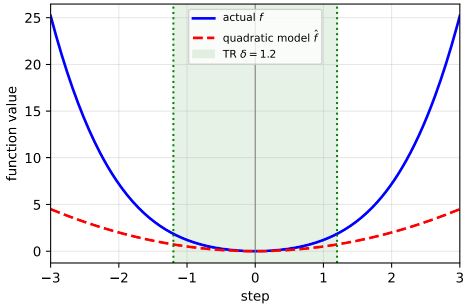
Good model: \eta > \eta_2 (expand TR)
