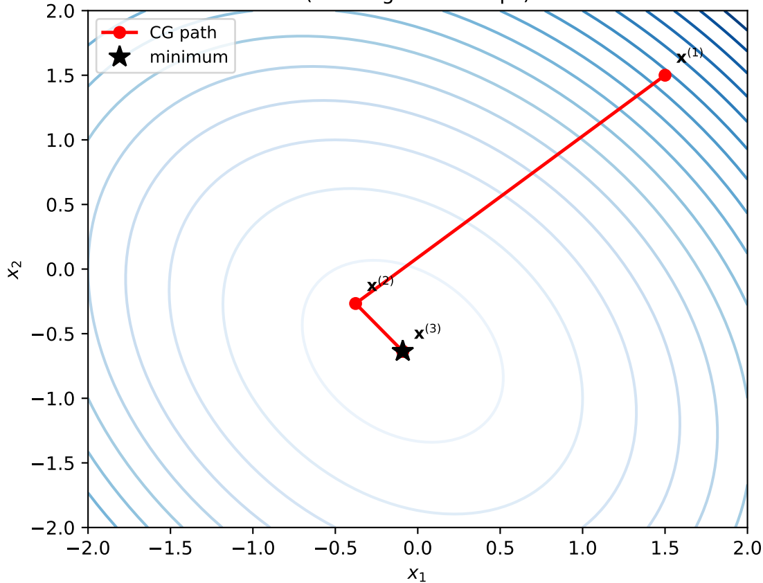
Conjugate Gradient on 2D Quadratic (converges in 2 steps)
