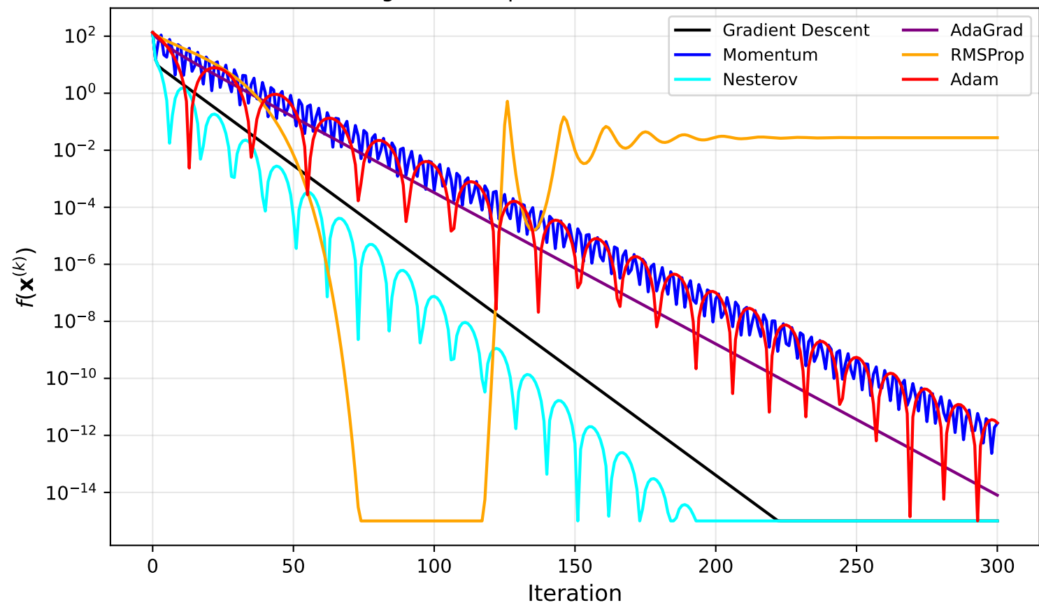
Convergence Comparison of First-Order Methods
