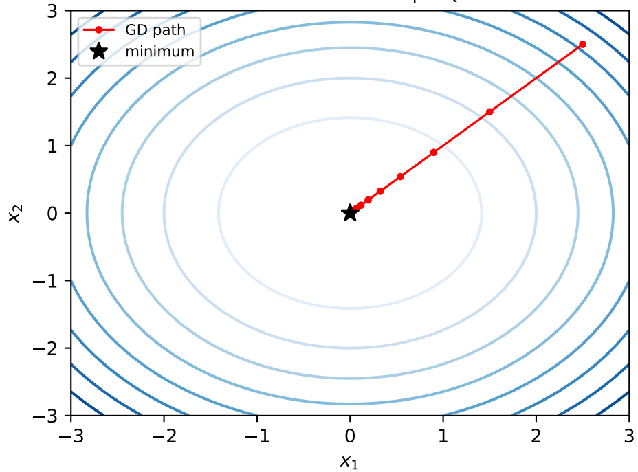
Gradient Descent on Isotropic Quadratic
