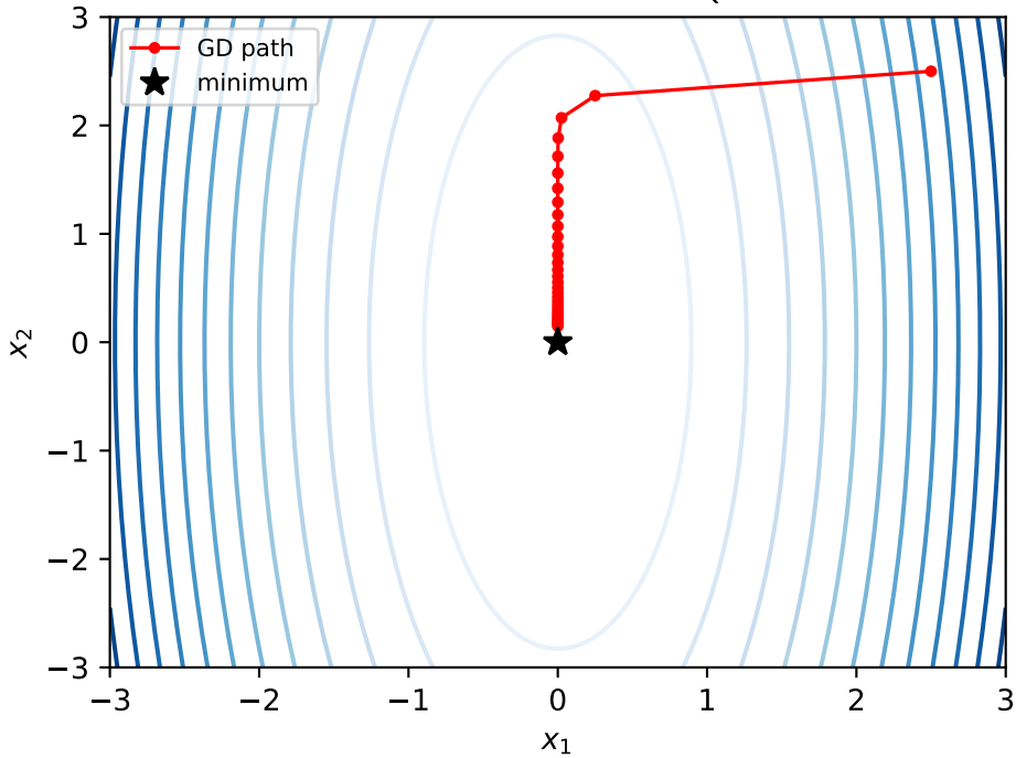
Gradient Descent on Narrow Quadratic
