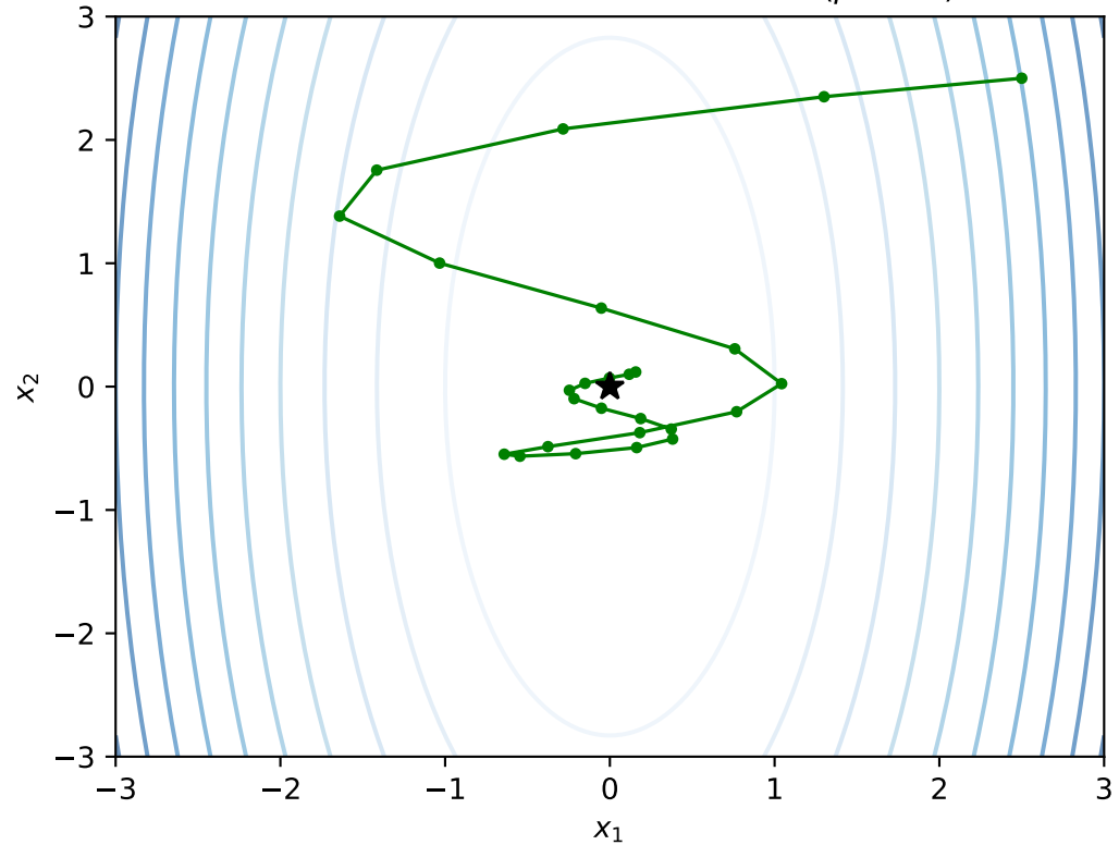
Gradient Descent with Momentum ( \beta = 0.8 )
