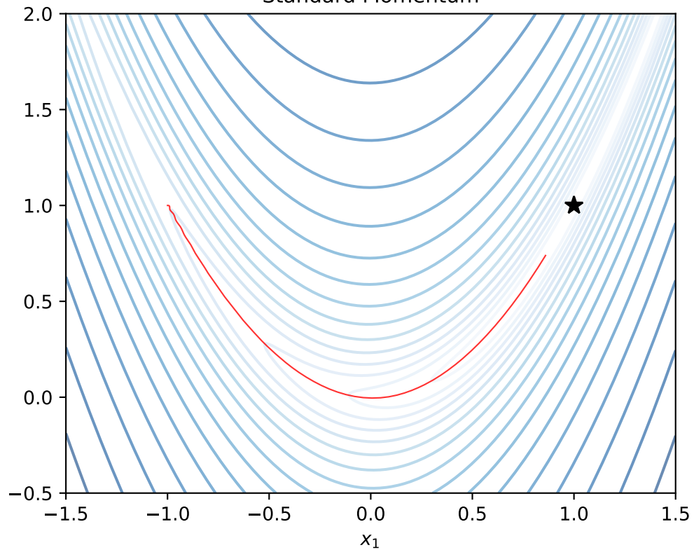
Standard Momentum
