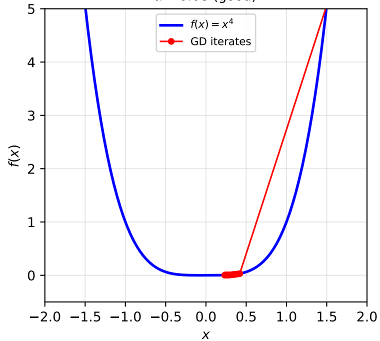
\alpha = 0.08 (good)
