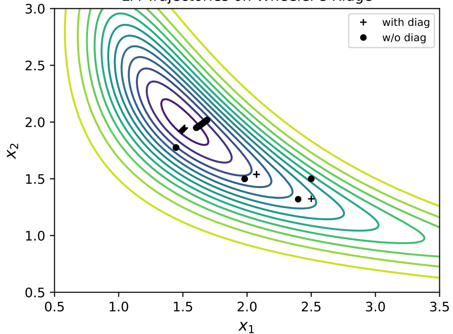
LM Trajectories on Wheeler's Ridge
