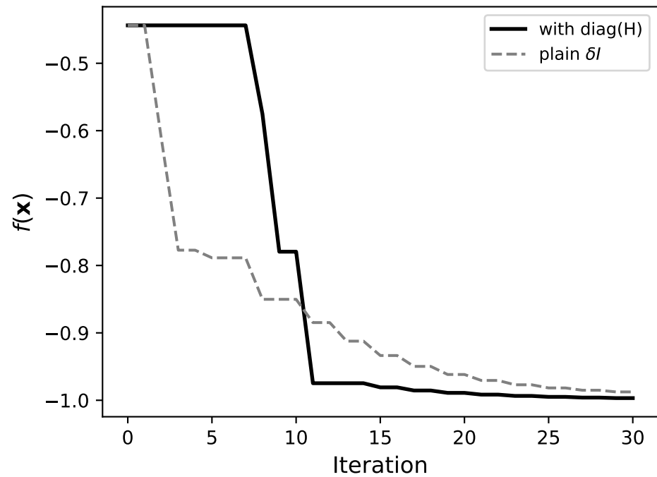
LM Convergence
