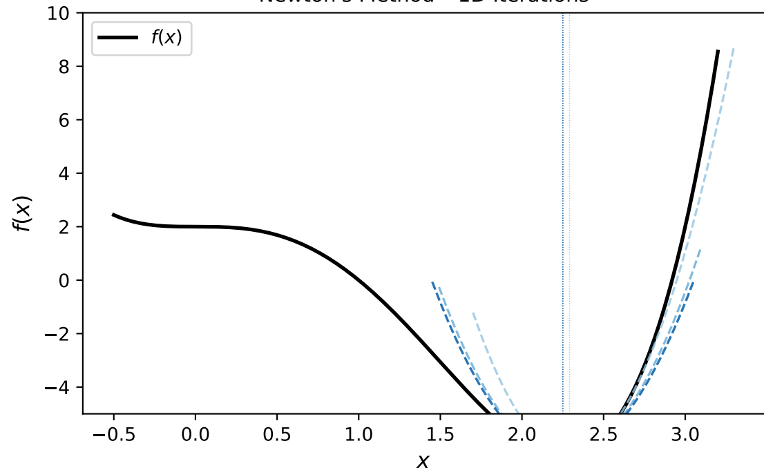
Newton's Method - 1D Iterations
