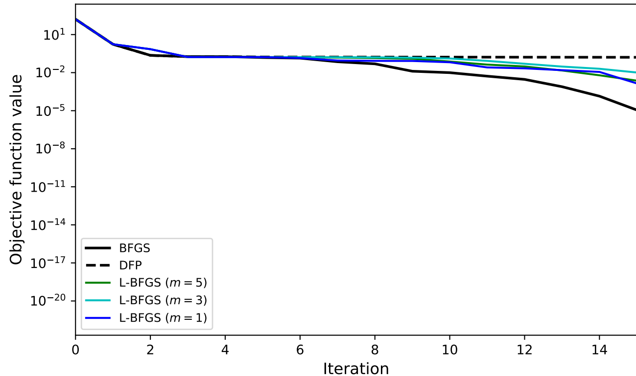
Quasi-Newton Methods: Rosenbrock (2D)
