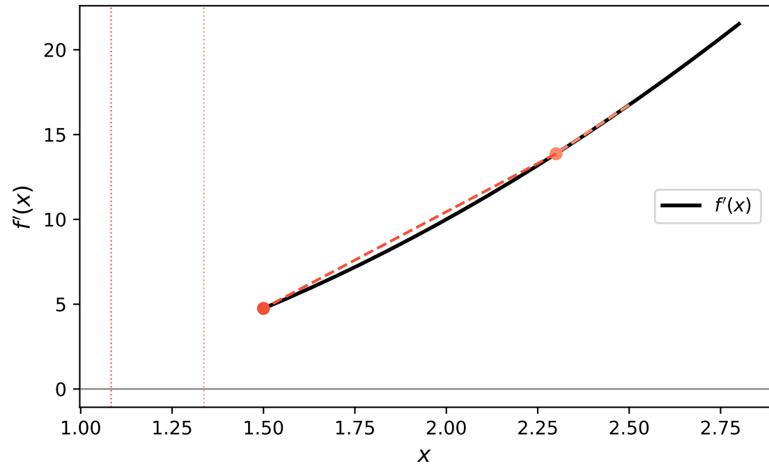
Secant Method: Approximating f'' from f'
