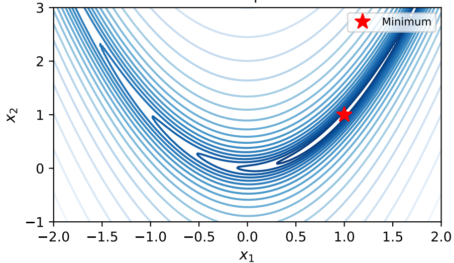
BFGS Update
