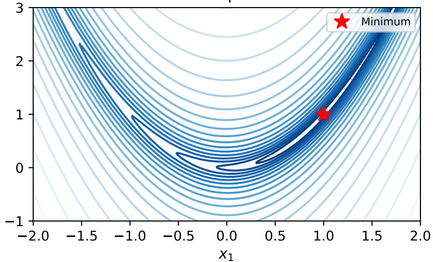
SR1 Update
