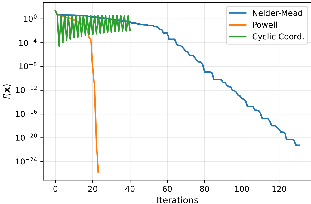
Convergence Comparison on Rosenbrock
