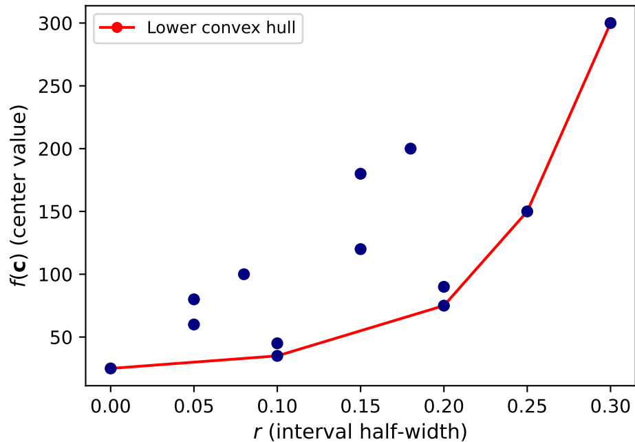
DIRECT: Potentially Optimal Intervals
