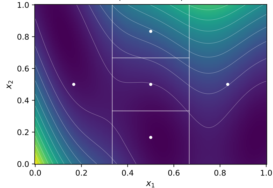
DIRECT: Interval Partitions (Branin function)
