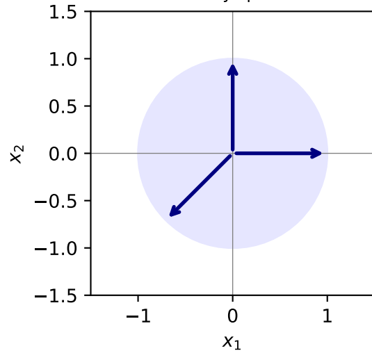
Positively spans \mathbb{R}^2
