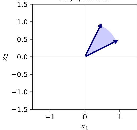
Only spans cone
