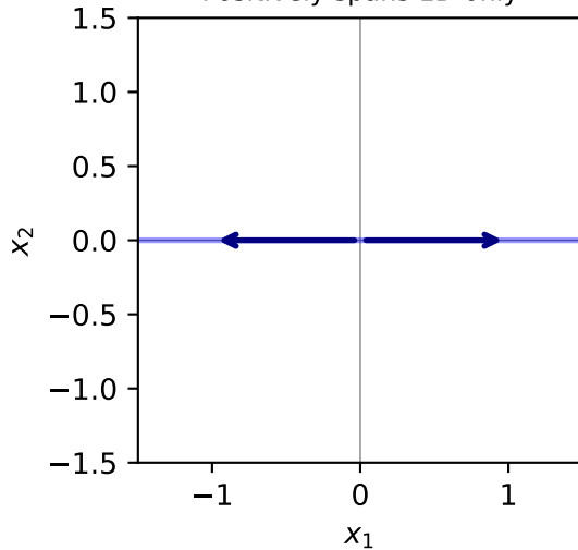
Positively spans 1D only
