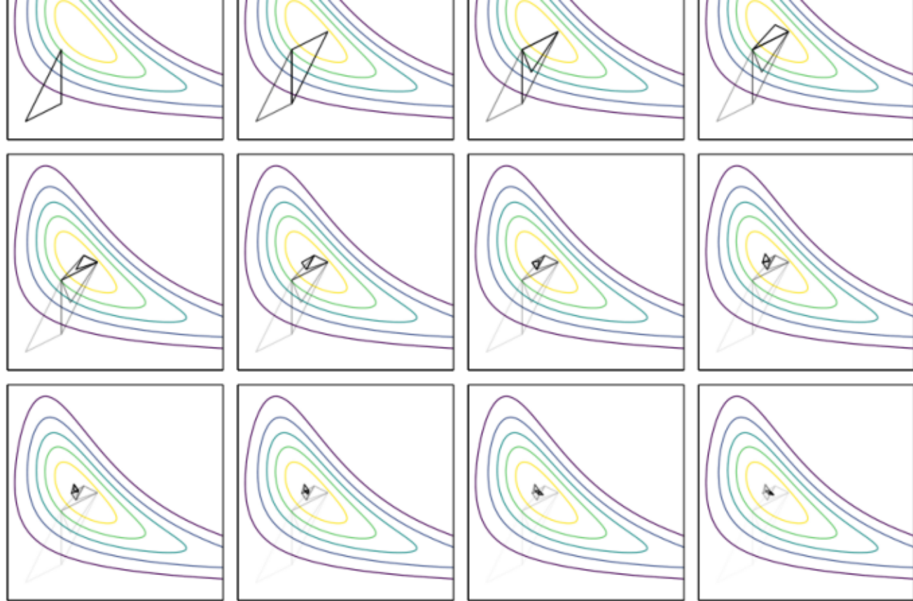
Figure 7.10. The Nelder-Mead method, proceeding left to right and top to bottom.
