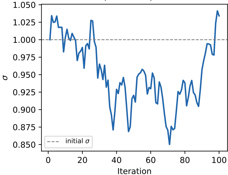
Step-Size \sigma Adaptation
