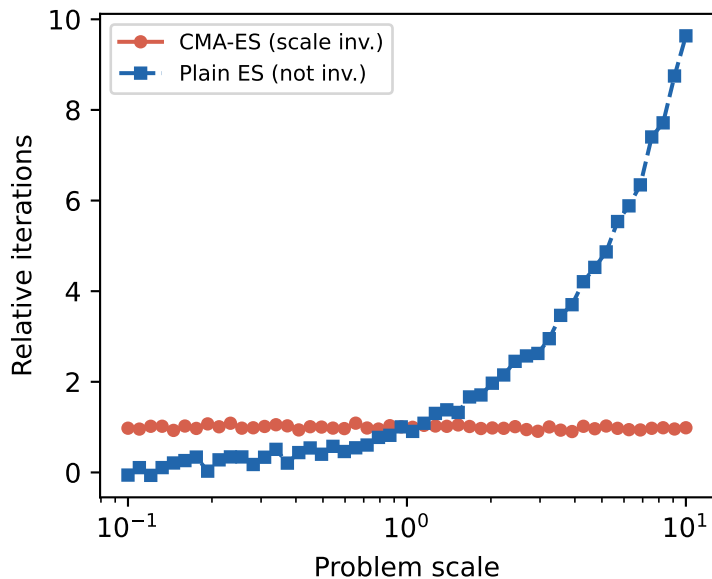
Scale Invariance of CMA-ES
