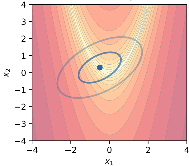
After 5 IGO steps
