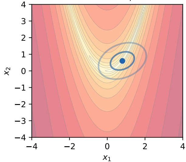
After 15 IGO steps
