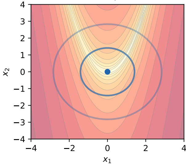
Initial \mathcal{N}(\mu, \Sigma)
