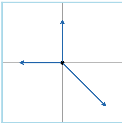
Positive Spanning Sets for \mathbb{R}^2 (Example 8.1)
