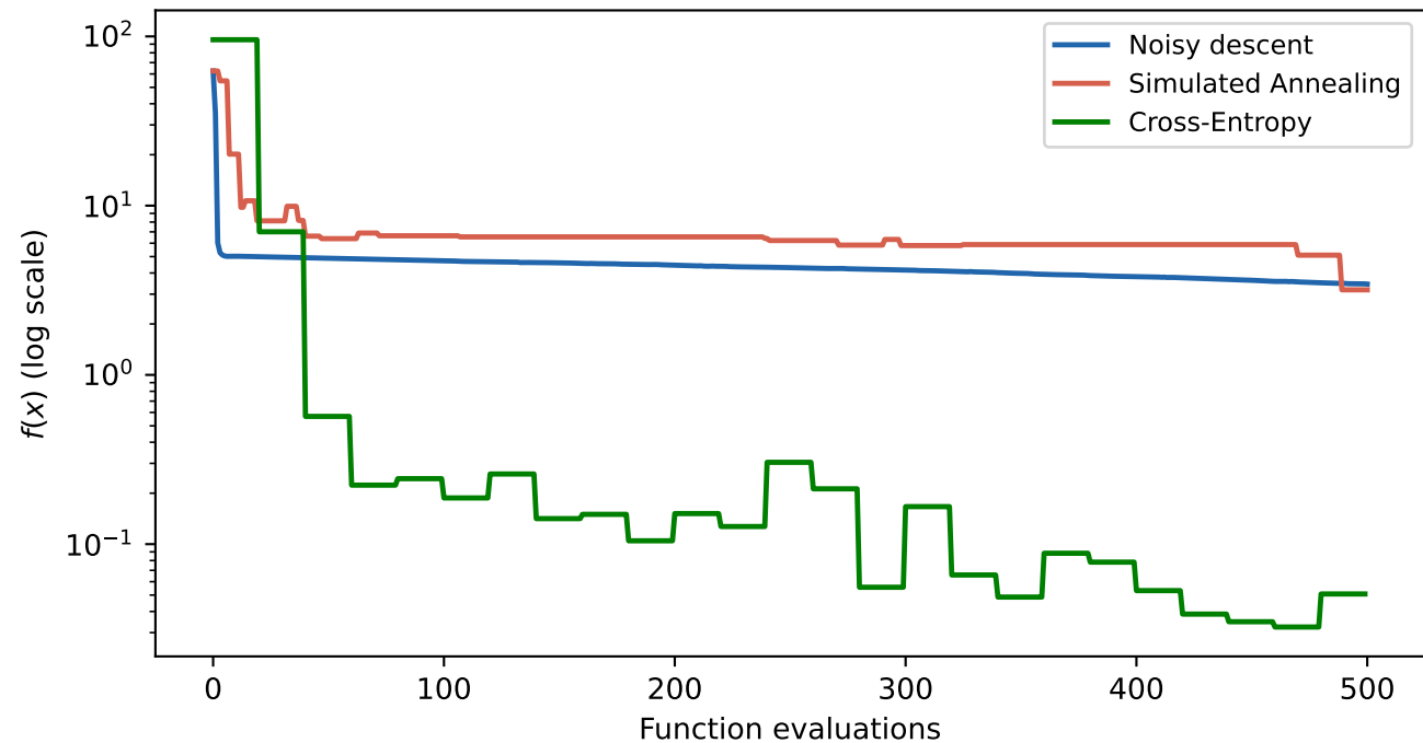
Method Comparison on Rosenbrock Function
