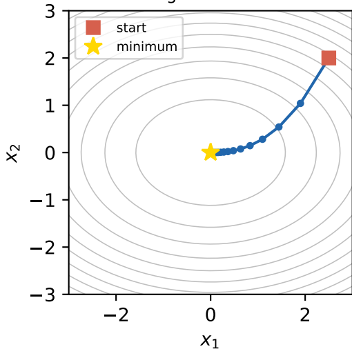
Clean gradient descent
