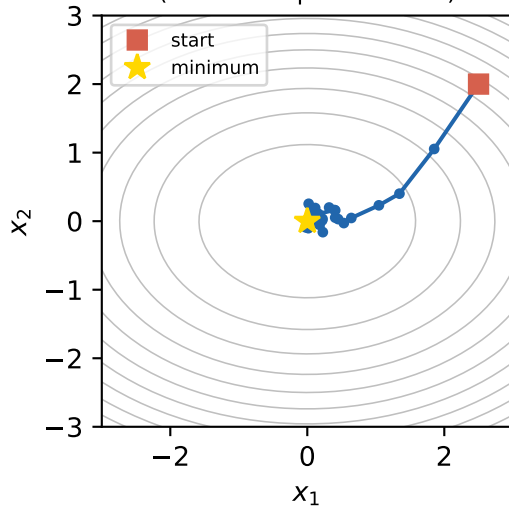
Noisy gradient descent (stochastic perturbation)
