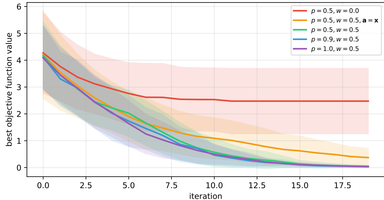
Differential Evolution Variants on Ackley's Function
