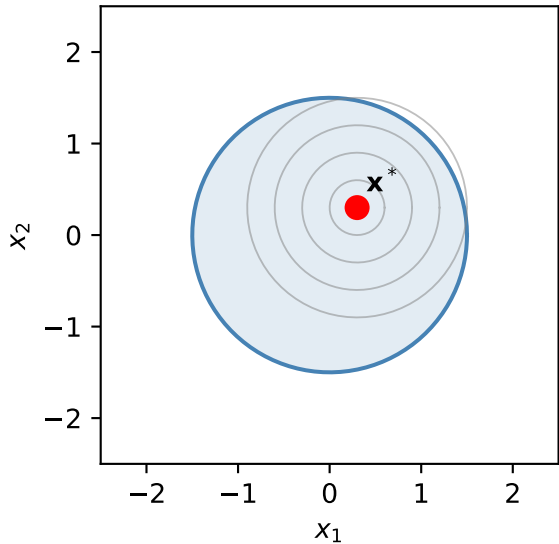
Inactive constraint g(\mathbf{x}^*) < 0
