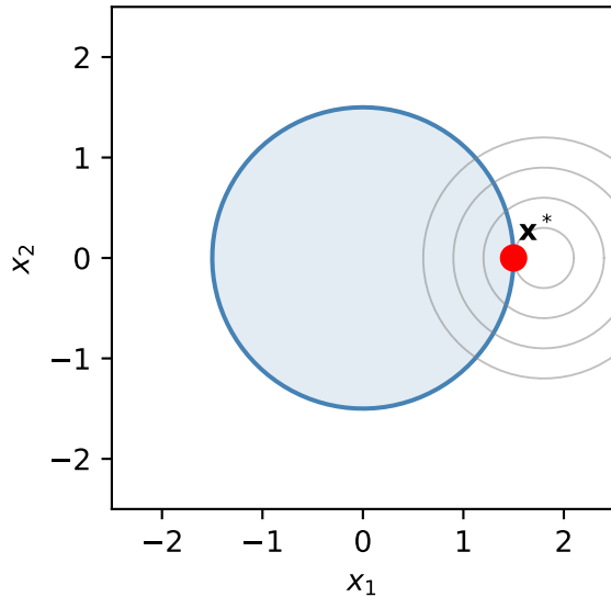
Active constraint g(\mathbf{x}^*) = 0
