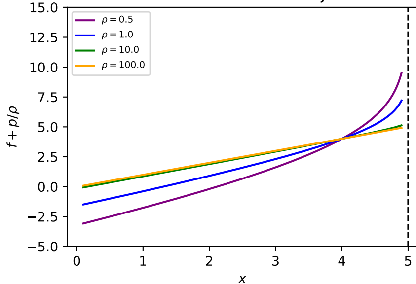
Interior Point Penalised Objective
