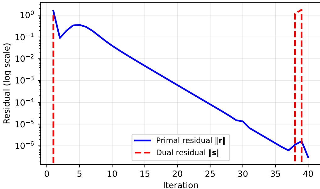
ADMM Convergence (Example 11.4)
