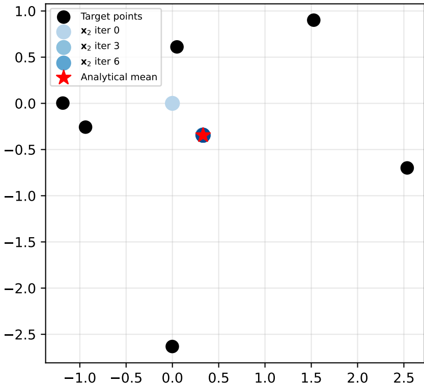
Consensus ADMM: Converging to Mean
