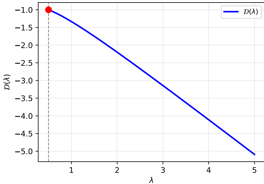
Dual Function \mathcal{D}(\lambda)
