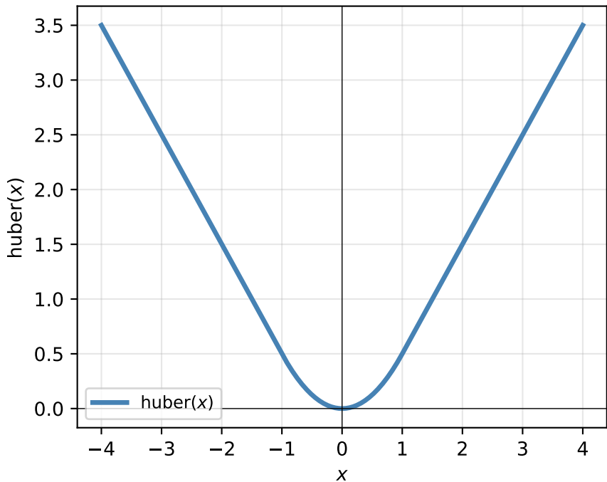
Huber Loss Function
