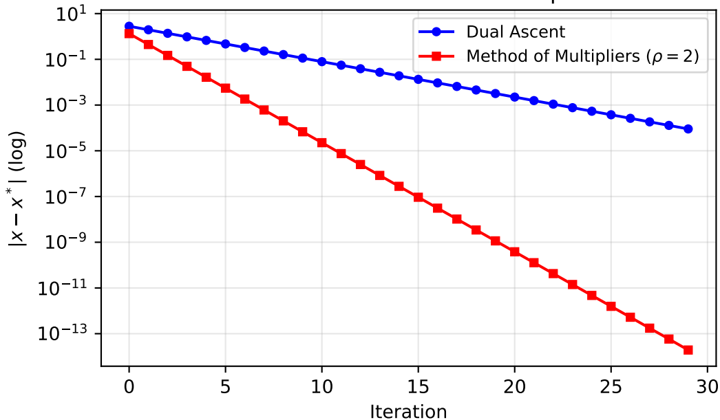
Dual Ascent vs Method of Multipliers
