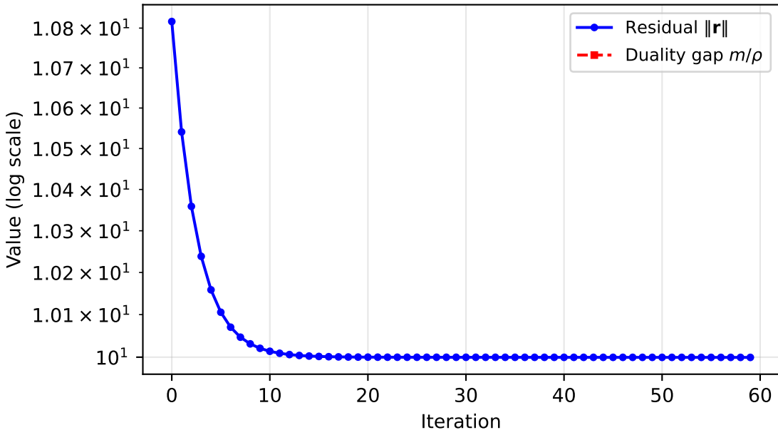
Primal-Dual Interior Point Convergence
