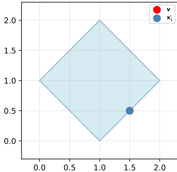
v inside \mathcal{X}
