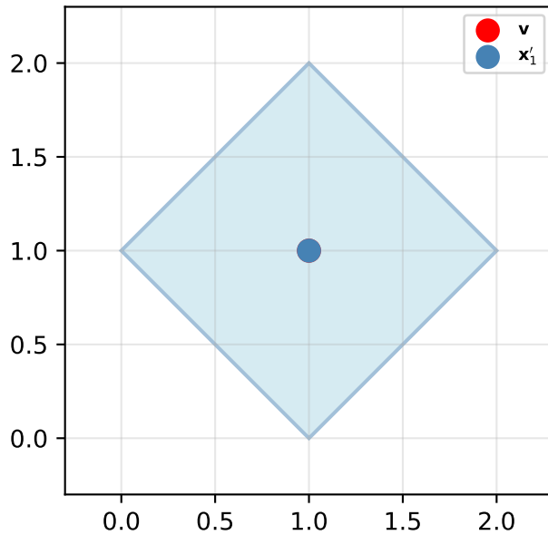
v on boundary
