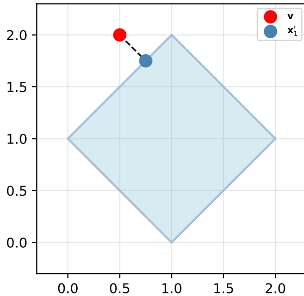
v outside \mathcal{X}
