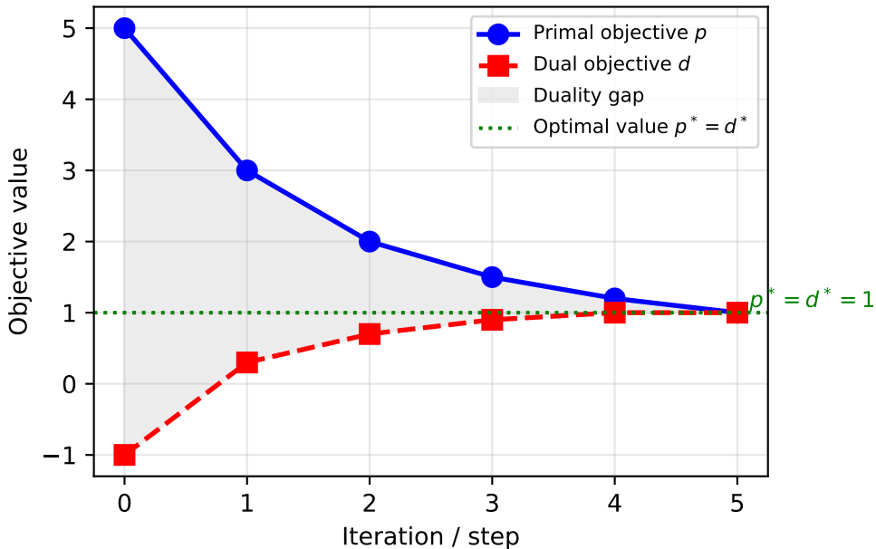
Strong Duality: Primal vs. Dual Objective
