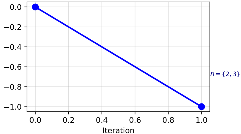
Objective Value per Simplex Iteration
