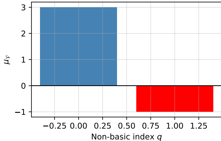
\mu_v at Initial Vertex (neg \Rightarrow suboptimal)
