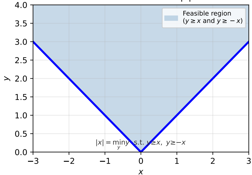
LP Reformulation of |x|
