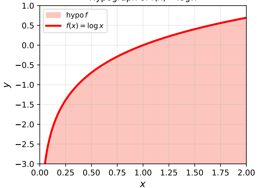
Hypograph of f(x) = \log x
