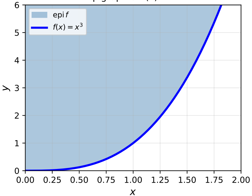
Epigraph of f(x) = x^3
