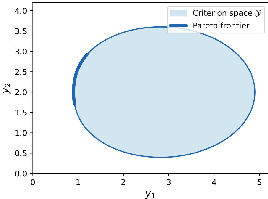
Criterion Space and Pareto Frontier
