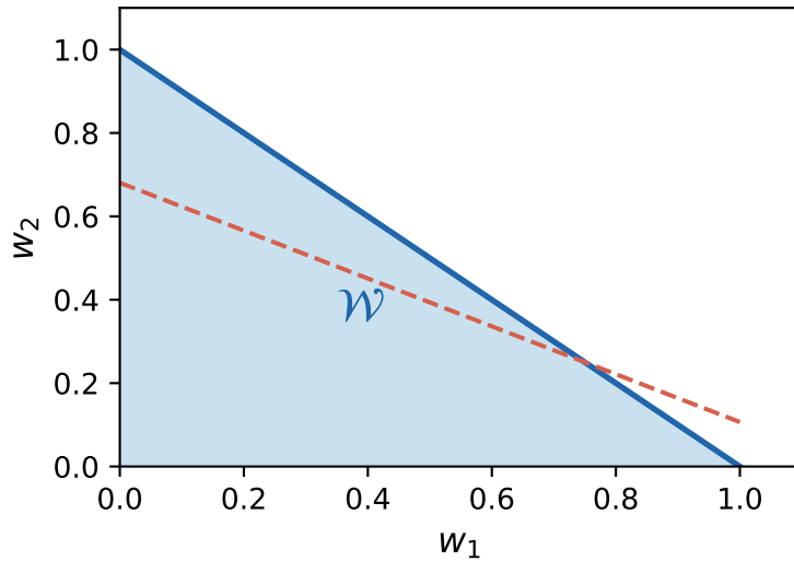
After 1 query
