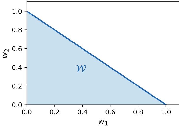
Initial \mathcal{W}
