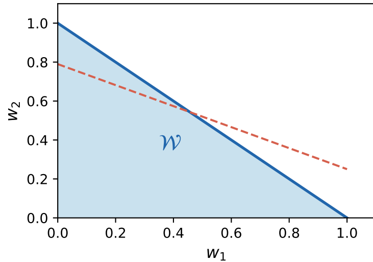
After 2 queries
