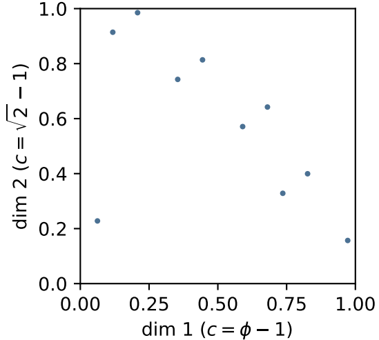
Additive Recurrence n=10
