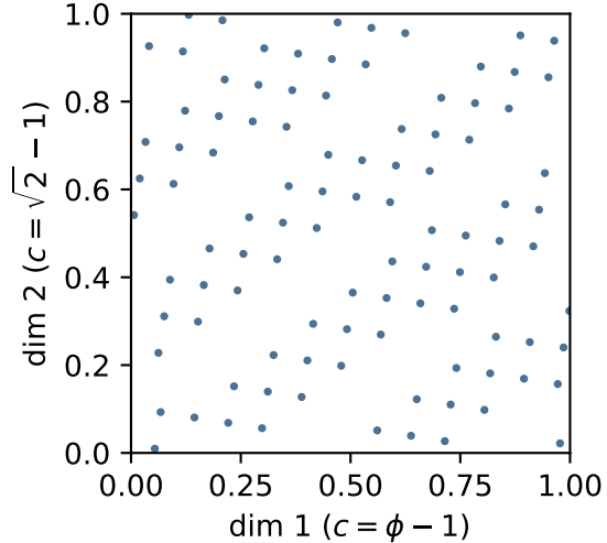
Additive Recurrence n=100
