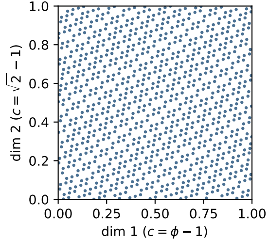
Additive Recurrence n=1000
