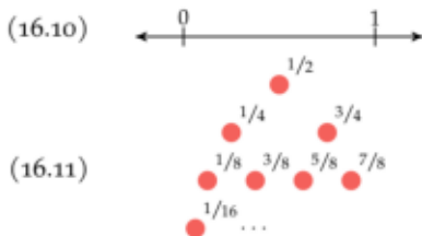
Figure 16.11. The first 8 values of the Halton sequence for b = 2 .
