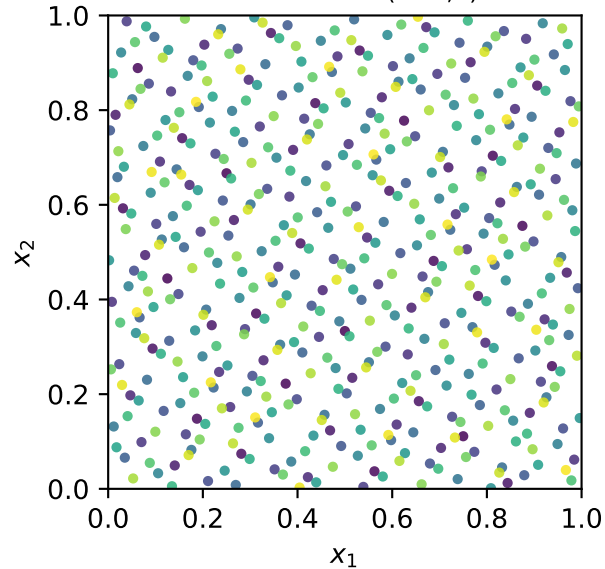
Halton n=500 (b=2,3)
