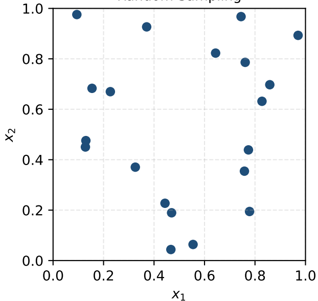
Random Sampling
