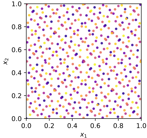
Sobol n=500
