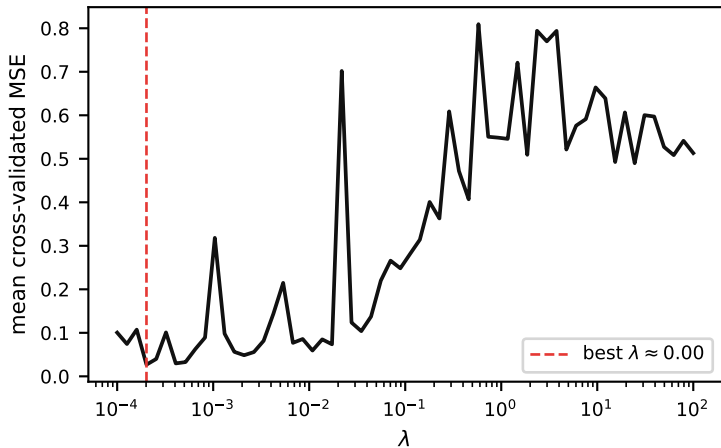
CV for Hyperparameter Selection
