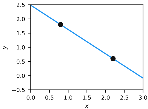
m = n + 1
