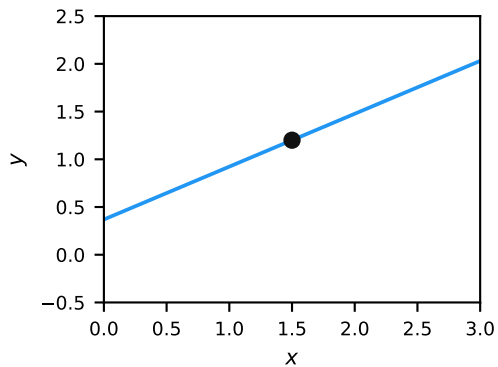
m < n + 1
