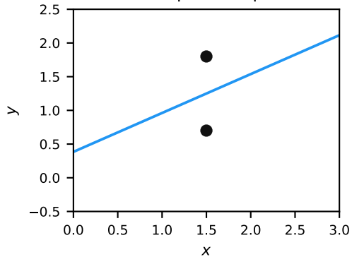
nonindependent points
