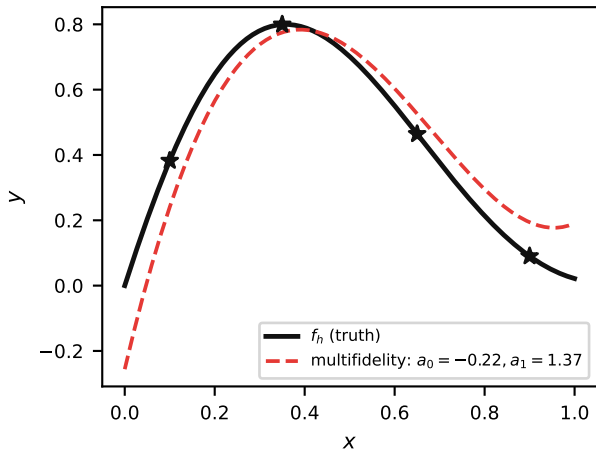
Multifidelity Surrogate
