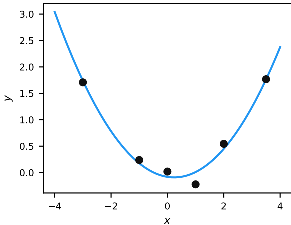
1-D polynomial fit
