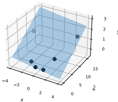
lifted to (x, x^2)
