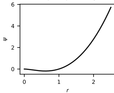
thin plate spline: r^2 \log r
