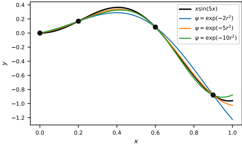
RBF Bandwidth Comparison (noise-free)
