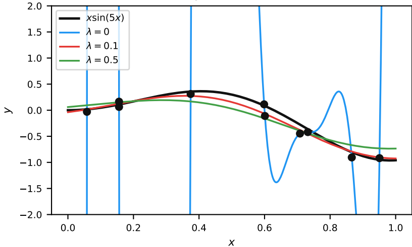
L_2 Regularisation Effect
